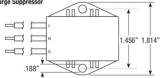
Surge Suppressor
