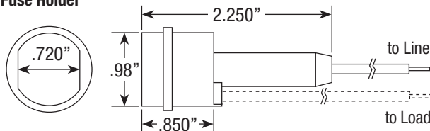
Fuse Holder
